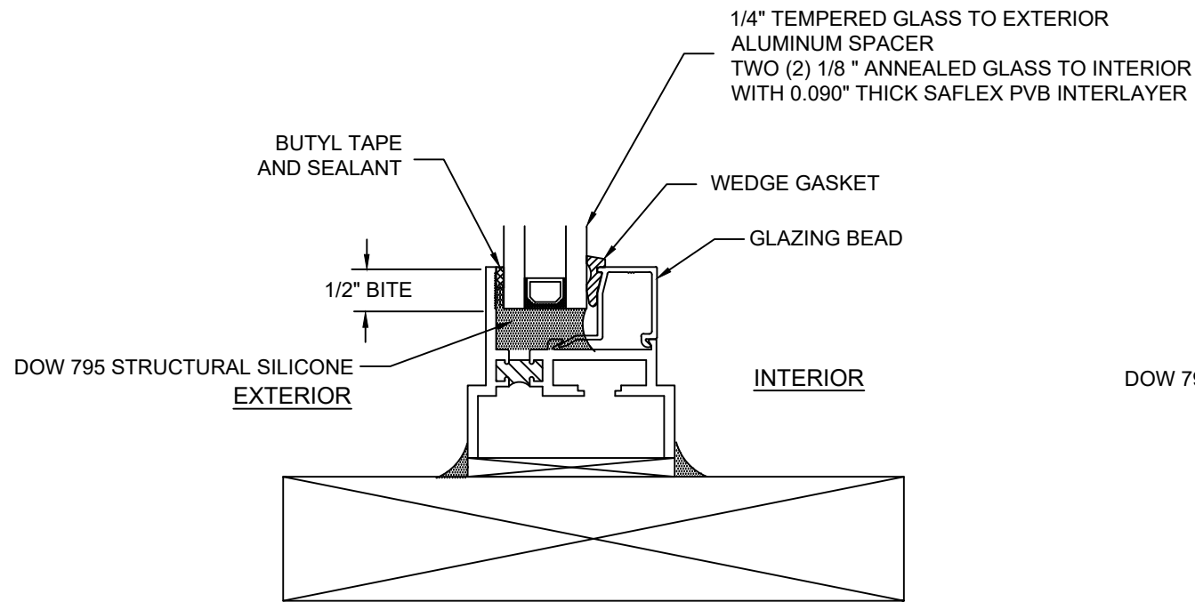
INSULATING GLASS GLAZING DETAIL
