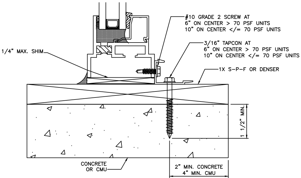
SECTION 1/1, 1/2 & 1/3 INSIDE CLIP & ANCHOR TO CONCRETE OR CMU WITH 1X BUCK STRIP
