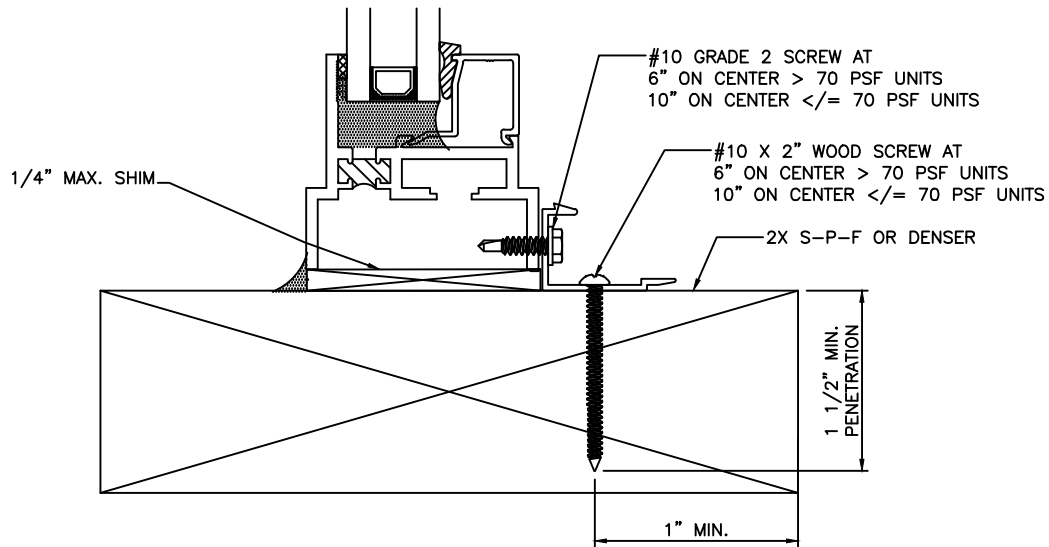
SECTION 1/1, 1/2 & 1/3 INSIDE CLIP & ANCHOR TO WOOD FRAME OR BUCK
