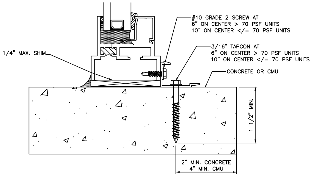
SECTION 1/1, 1/2 & 1/3 INSIDE CLIP & ANCHOR TO CONCRETE OR CMU
