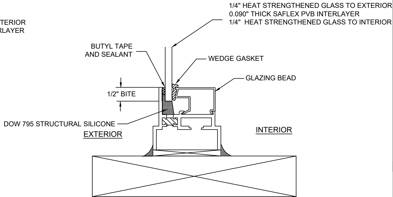
MONOLITHIC GLASS GLAZING DETAIL
