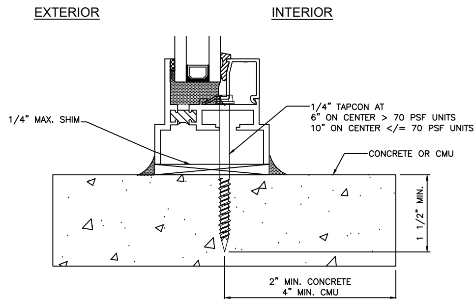
SECTION 1/1, 1/2 & 1/3 THROUGH FRAME TO CONCRETE OR CMU
